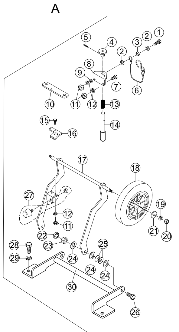
Figure 1. WHL88TKit Parts
